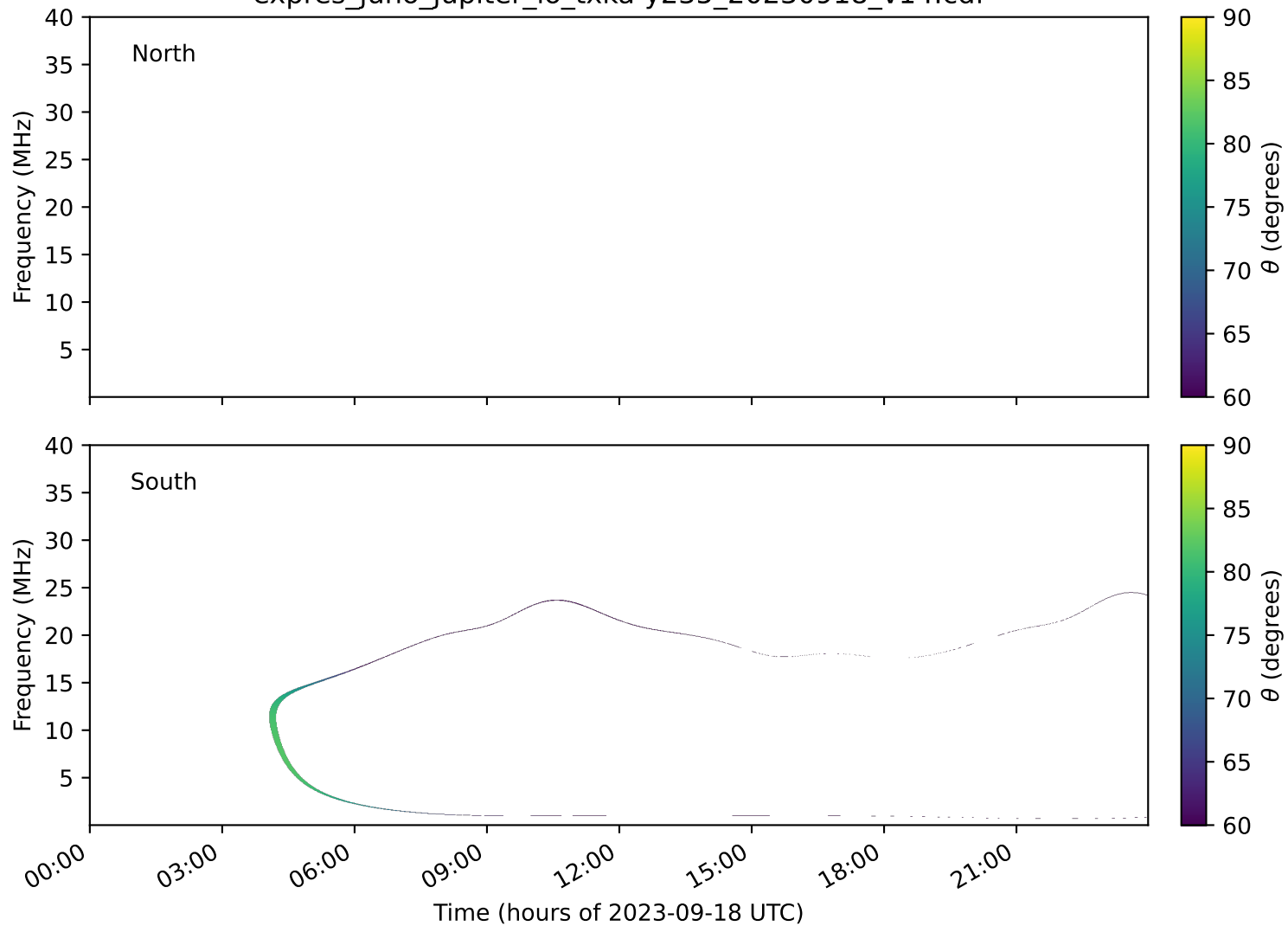
expres_juno_jupiter_io_txka-y235_20230918_v14.cdf
