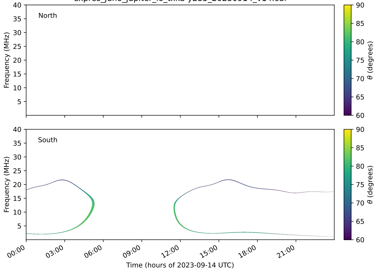
expres_juno_jupiter_io_txka-y235_20230914_v14.cdf
