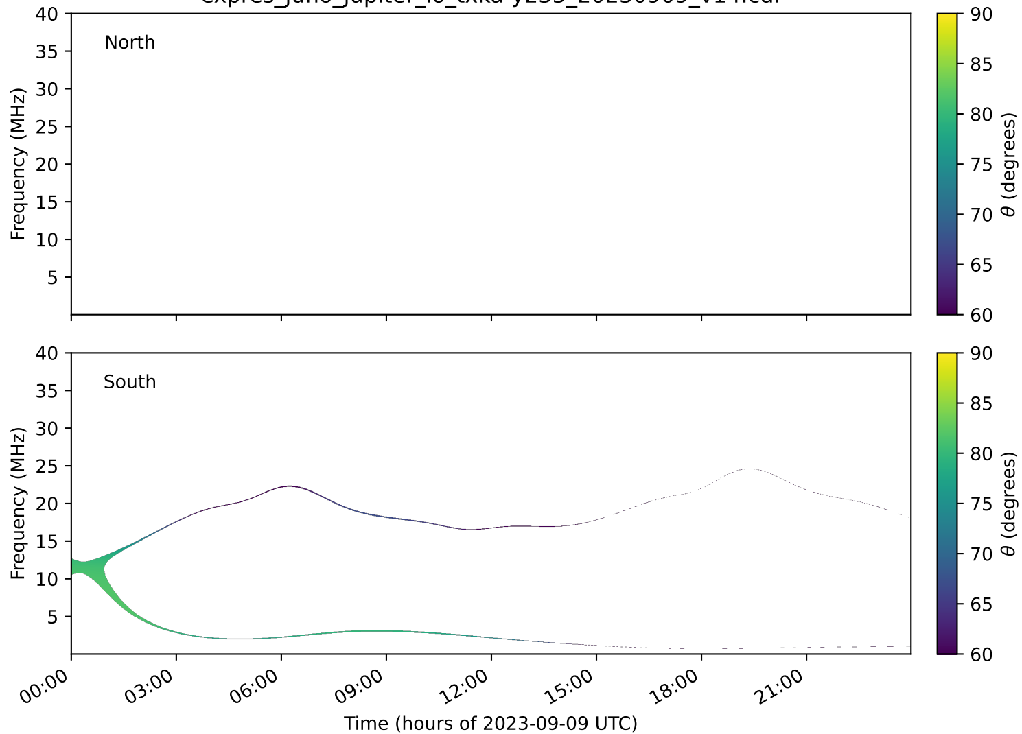
expres_juno_jupiter_io_txka-y235_20230909_v14.cdf
