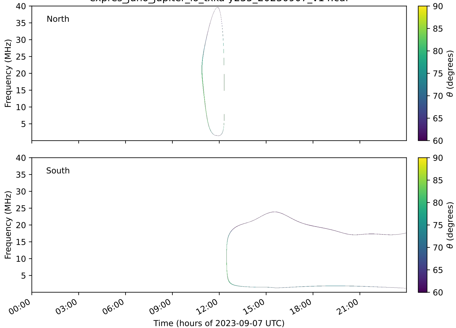
expres_juno_jupiter_io_txka-y235_20230907_v14.cdf
