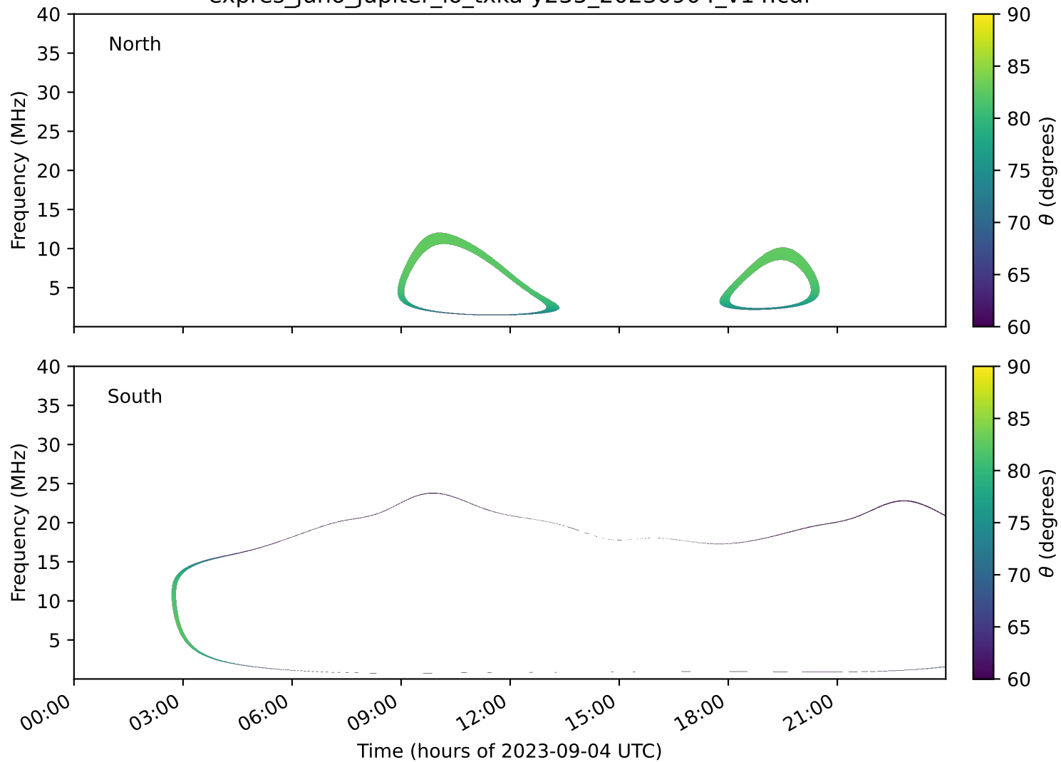
expres_juno_jupiter_io_txka-y235_20230904_v14.cdf
