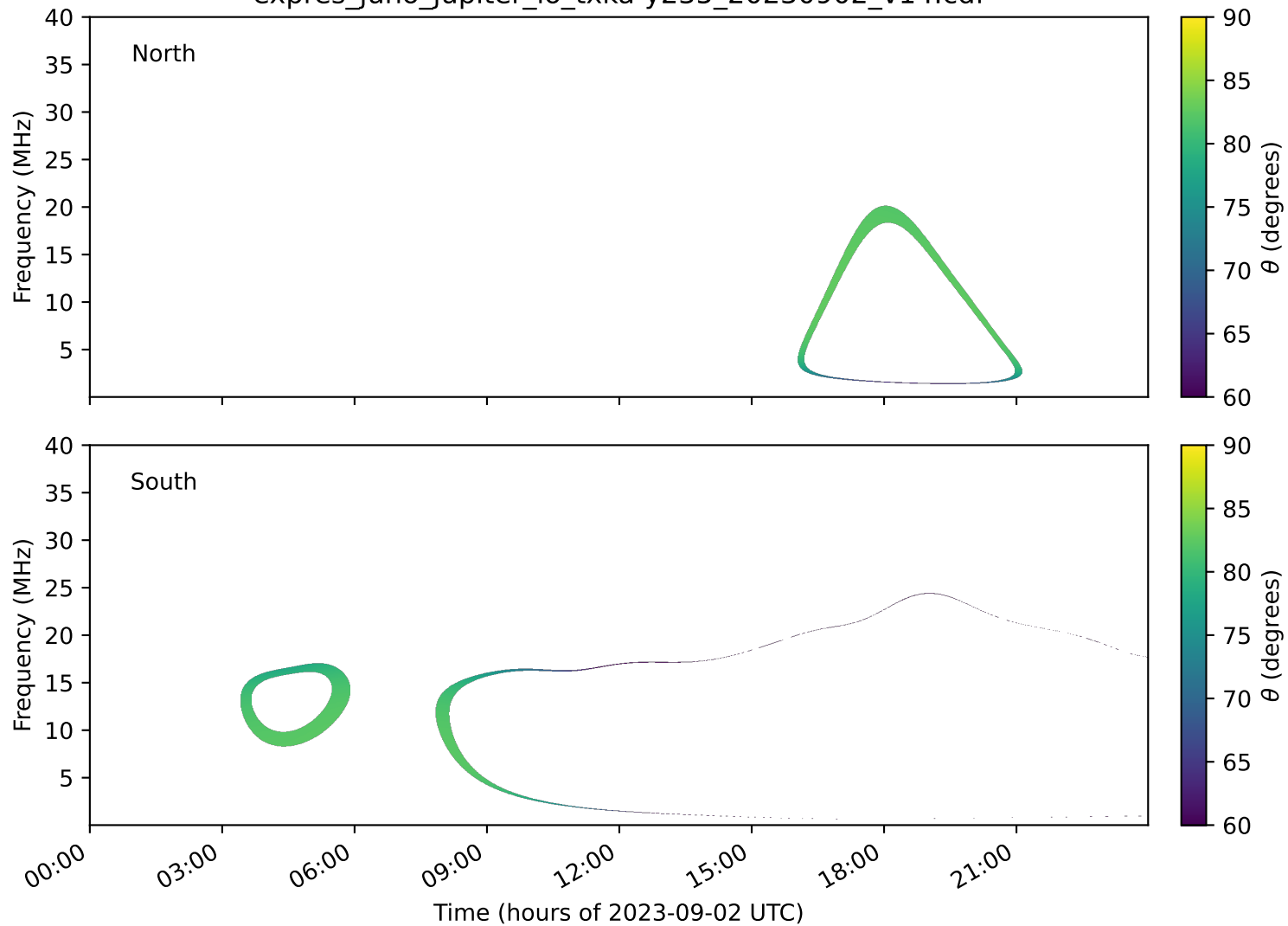
expres_juno_jupiter_io_txka-y235_20230902_v14.cdf
