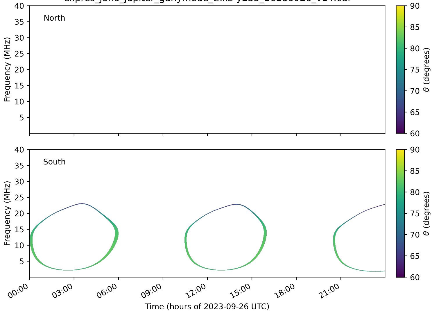
expres_juno_jupiter_ganymede_txka-y235_20230926_v14.cdf
