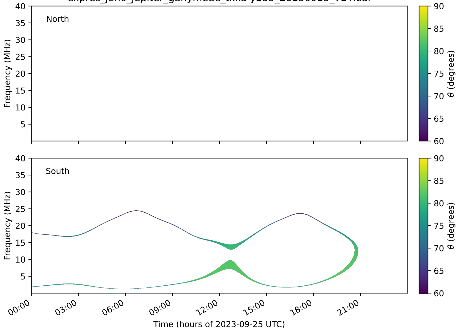
expres_juno_jupiter_ganymede_txka-y235_20230925_v14.cdf
