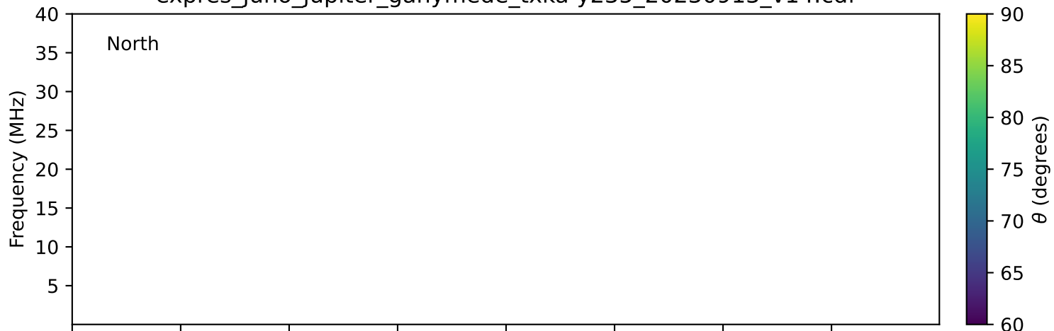
expres_juno_jupiter_ganymede_txka-y235_20230913_v14.cdf
