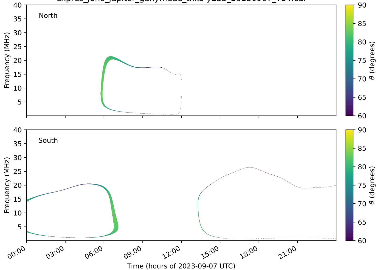
expres_juno_jupiter_ganymede_txka-y235_20230907_v14.cdf
