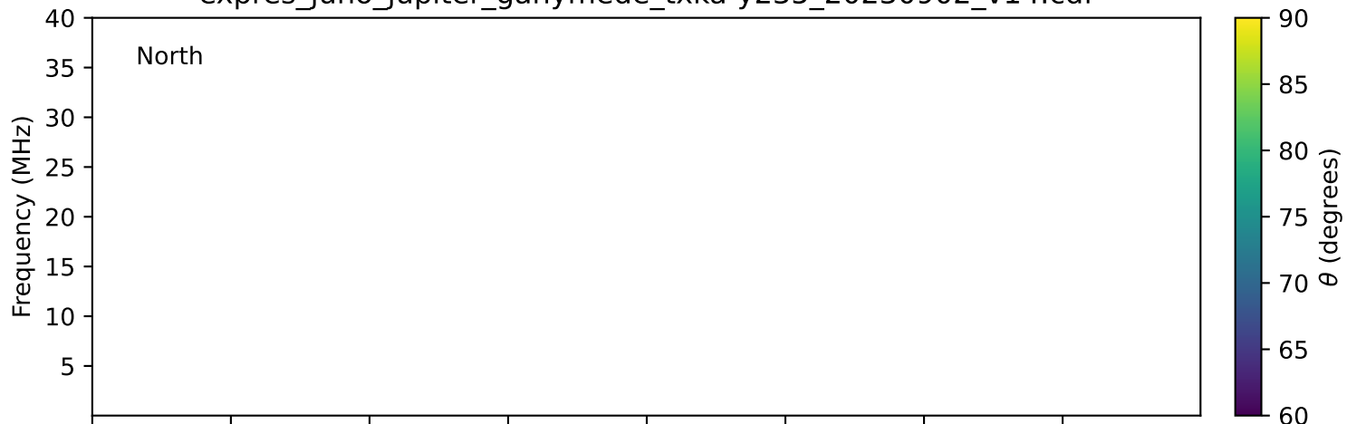
expres_juno_jupiter_ganymede_txka-y235_20230902_v14.cdf
