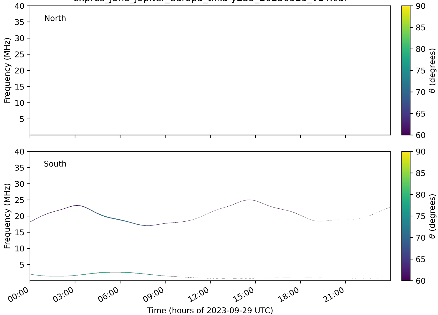
expres_juno_jupiter_europa_txka-y235_20230929_v14.cdf
