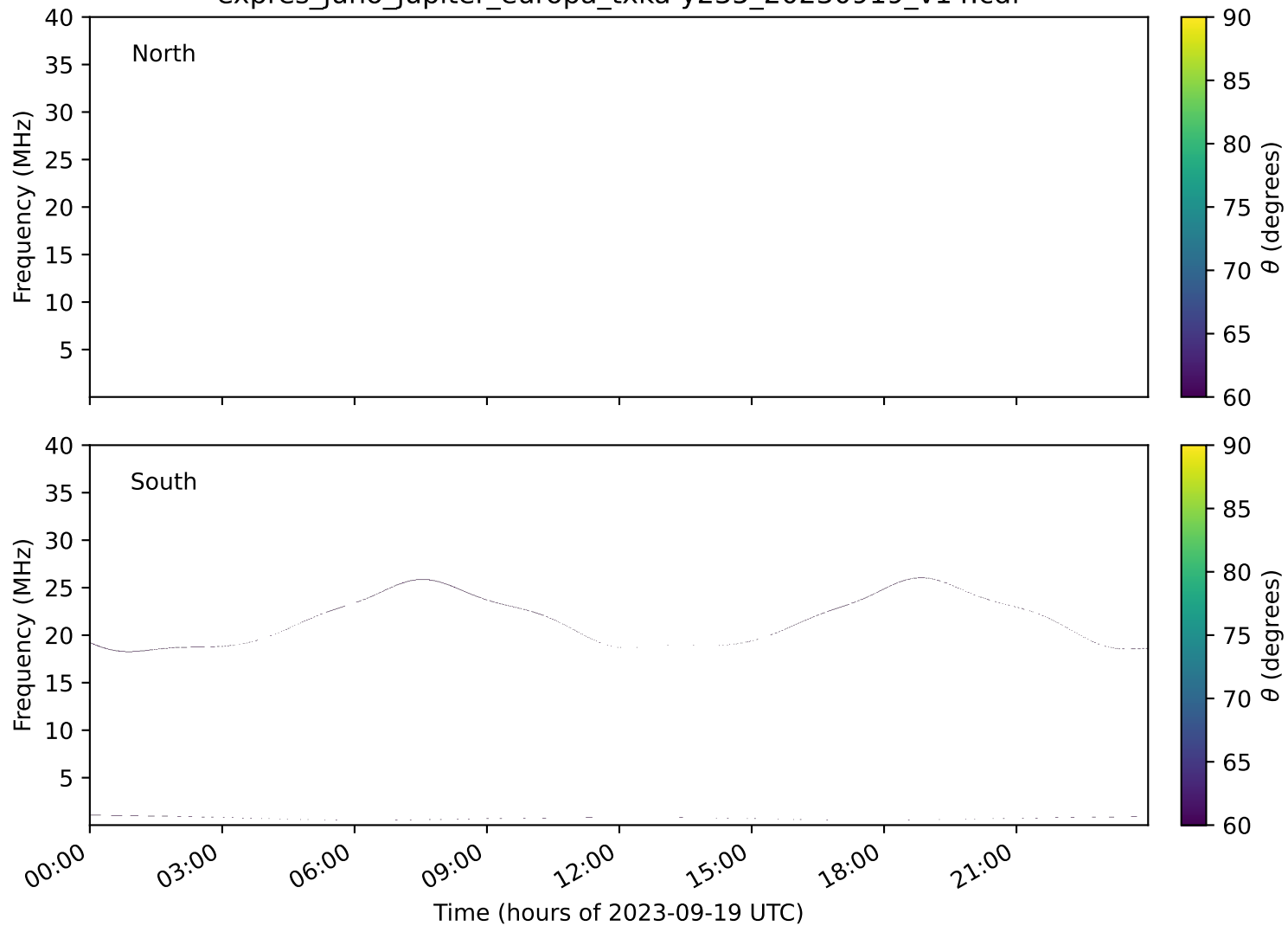
expres_juno_jupiter_europa_txka-y235_20230919_v14.cdf
