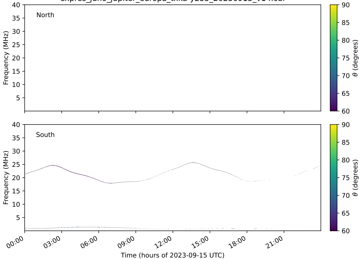
expres_juno_jupiter_europa_txka-y235_20230915_v14.cdf
