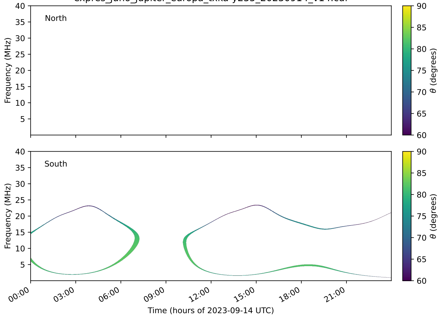
expres_juno_jupiter_europa_txka-y235_20230914_v14.cdf
