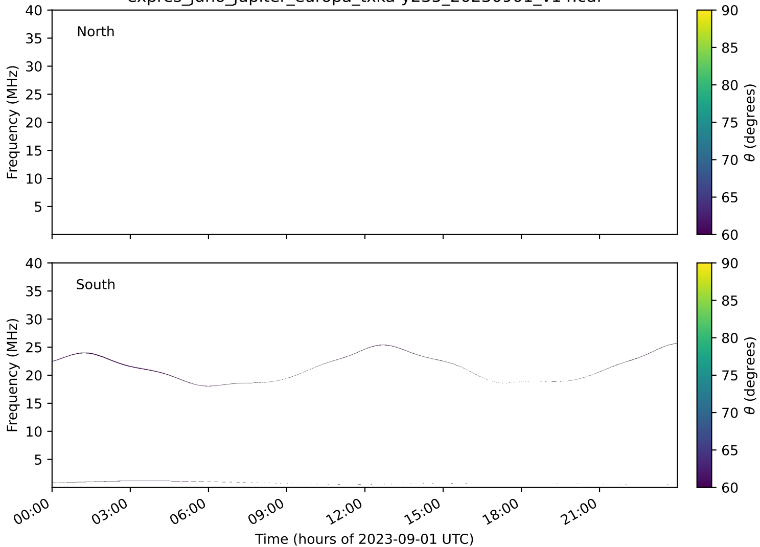
expres_juno_jupiter_europa_txka-y235_20230901_v14.cdf
