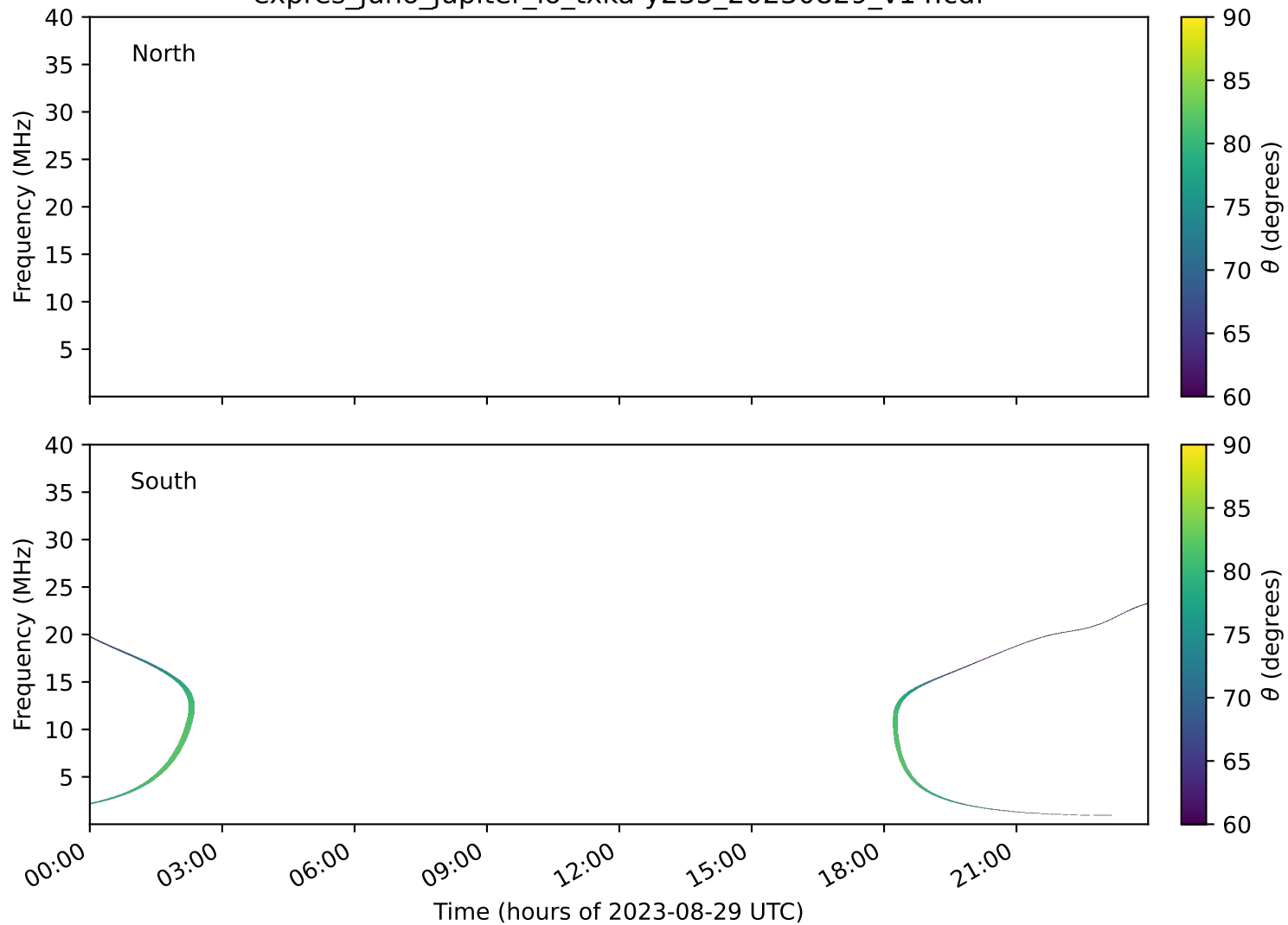
expres_juno_jupiter_io_txka-y235_20230829_v14.cdf
