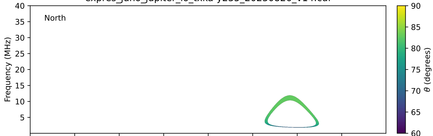
expres_juno_jupiter_io_txka-y235_20230826_v14.cdf
