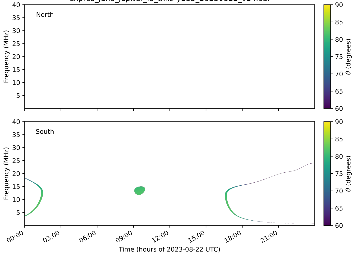
expres_juno_jupiter_io_txka-y235_20230822_v14.cdf
