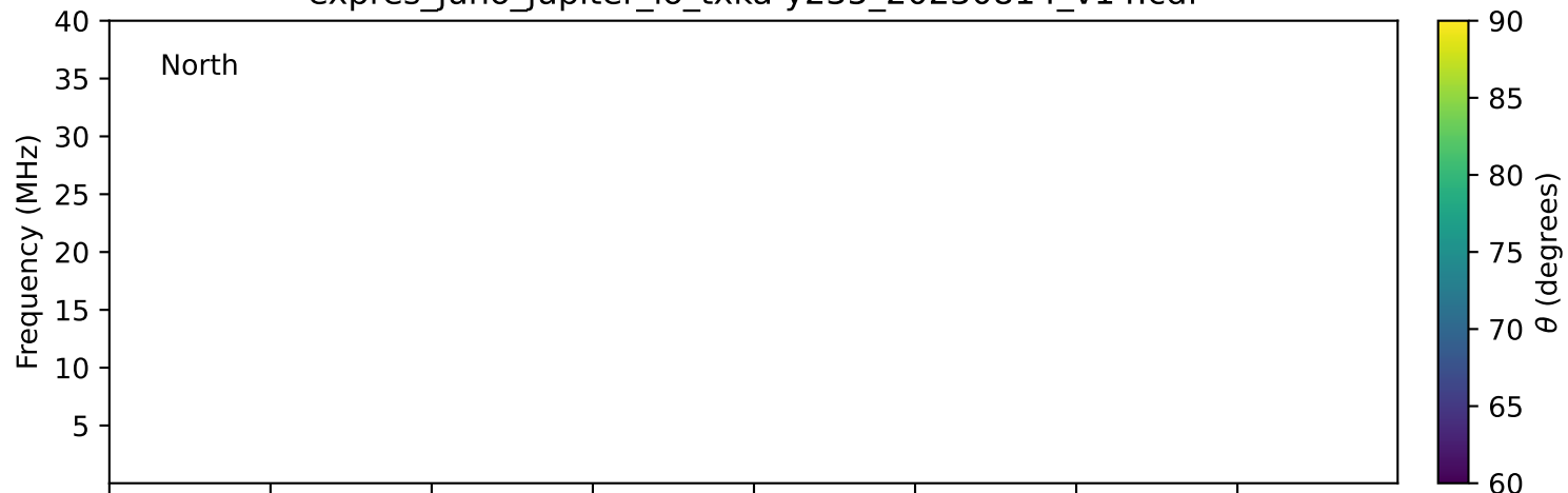
expres_juno_jupiter_io_txka-y235_20230814_v14.cdf
