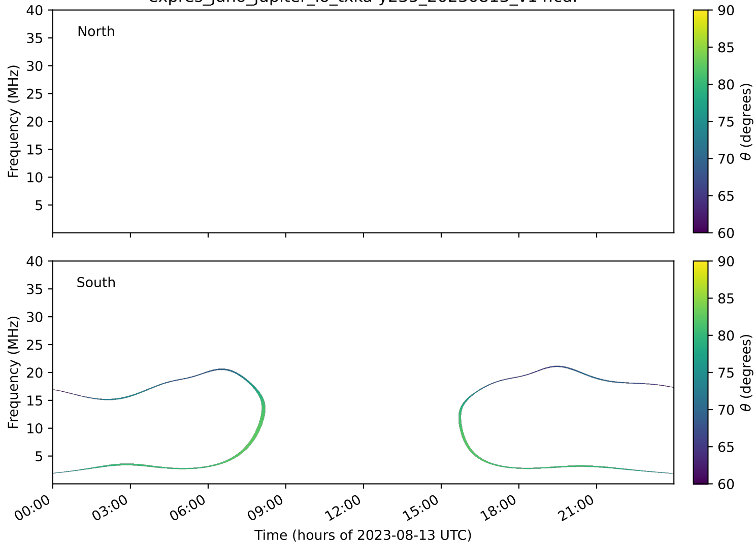
expres_juno_jupiter_io_txka-y235_20230813_v14.cdf
