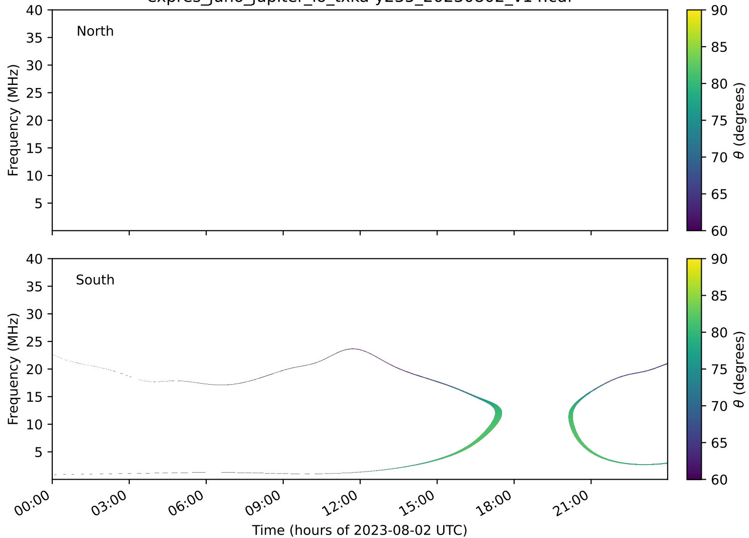
expres_juno_jupiter_io_txka-y235_20230802_v14.cdf
