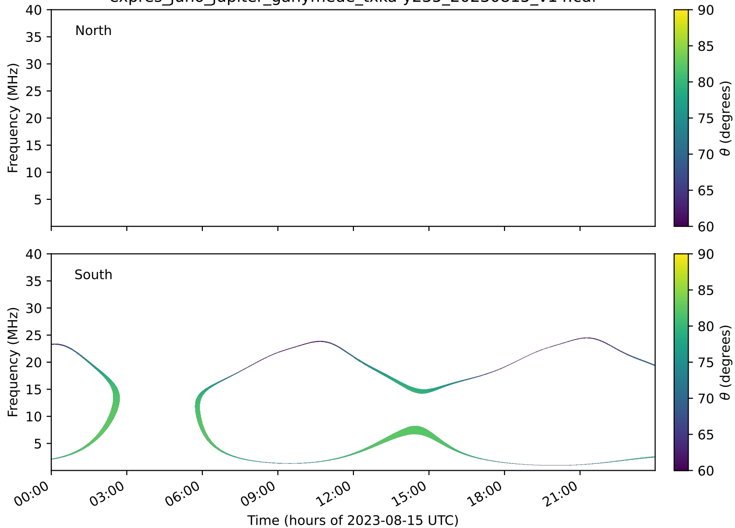
expres_juno_jupiter_ganymede_txka-y235_20230815_v14.cdf
