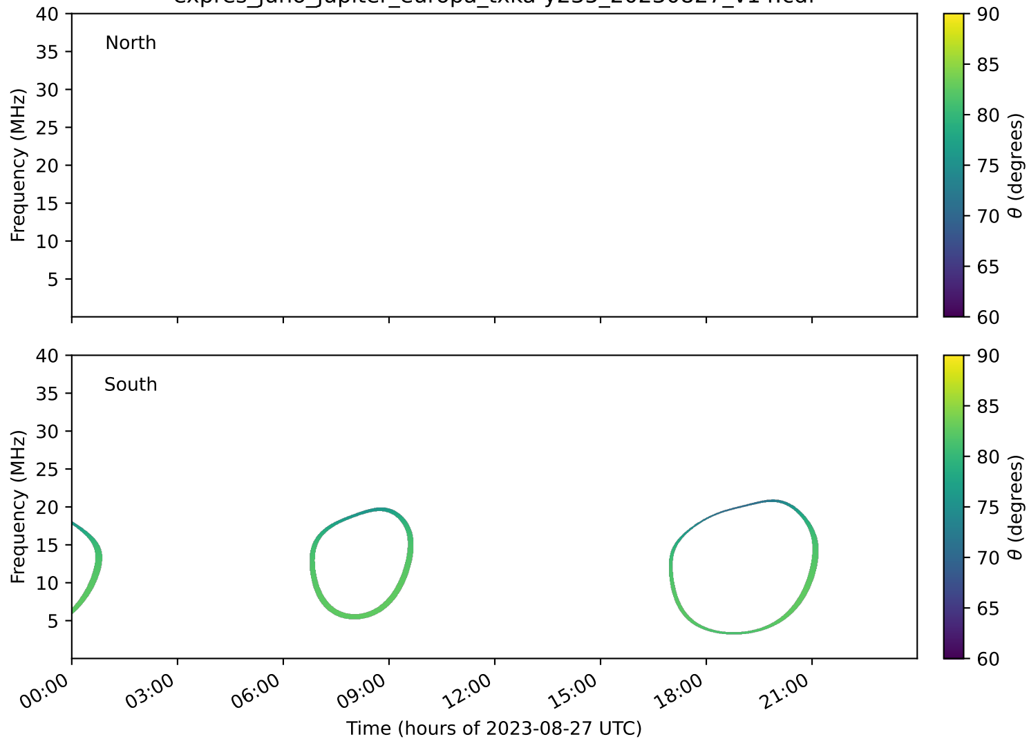
expres_juno_jupiter_europa_txka-y235_20230827_v14.cdf
