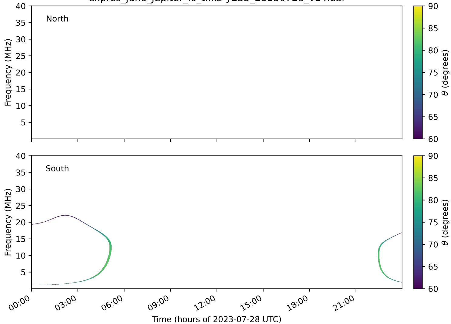
expres_juno_jupiter_io_txka-y235_20230728_v14.cdf
