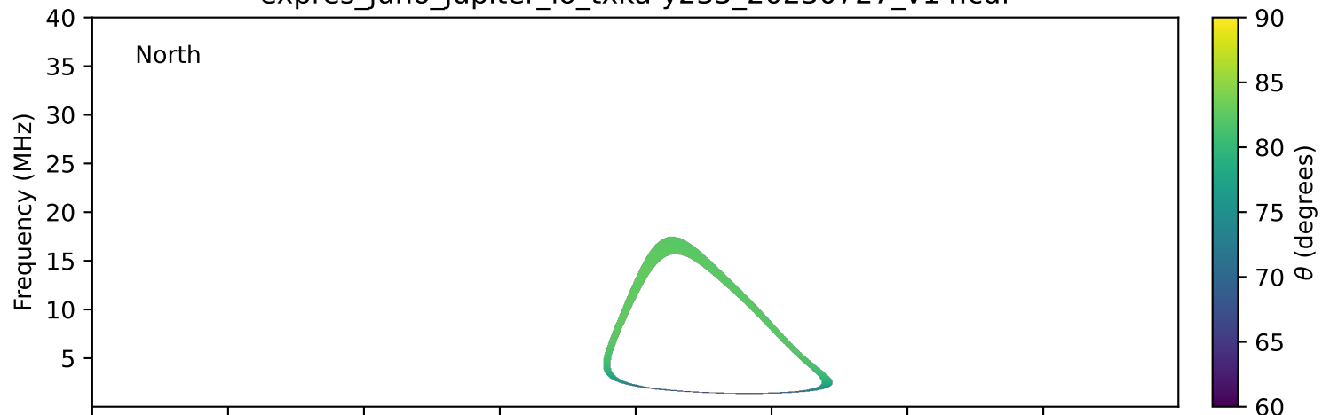
expres_juno_jupiter_io_txka-y235_20230727_v14.cdf
