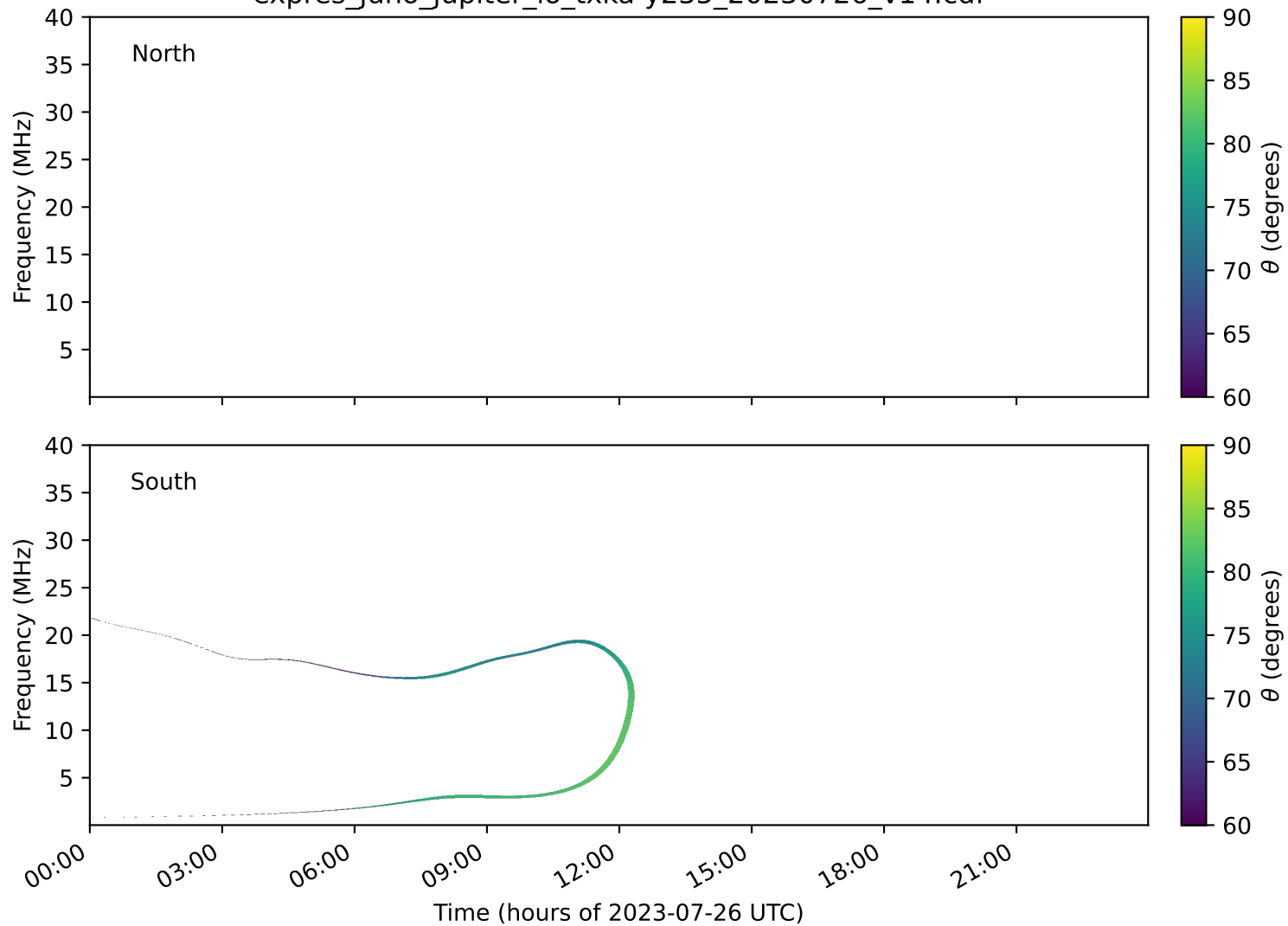
expres_juno_jupiter_io_txka-y235_20230726_v14.cdf
