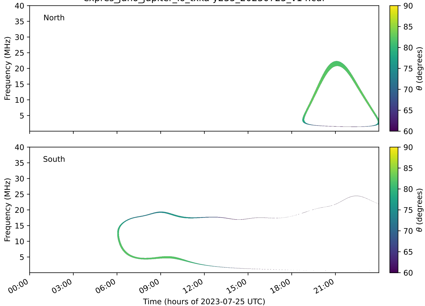
expres_juno_jupiter_io_txka-y235_20230725_v14.cdf
