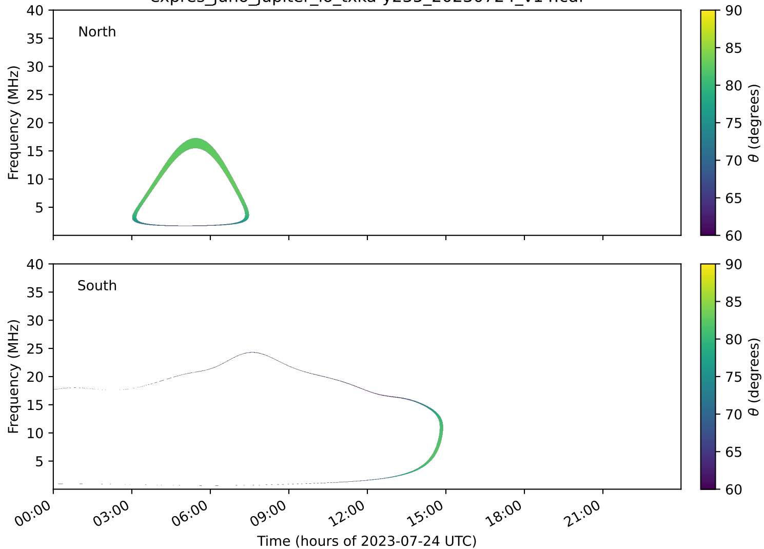
expres_juno_jupiter_io_txka-y235_20230724_v14.cdf
