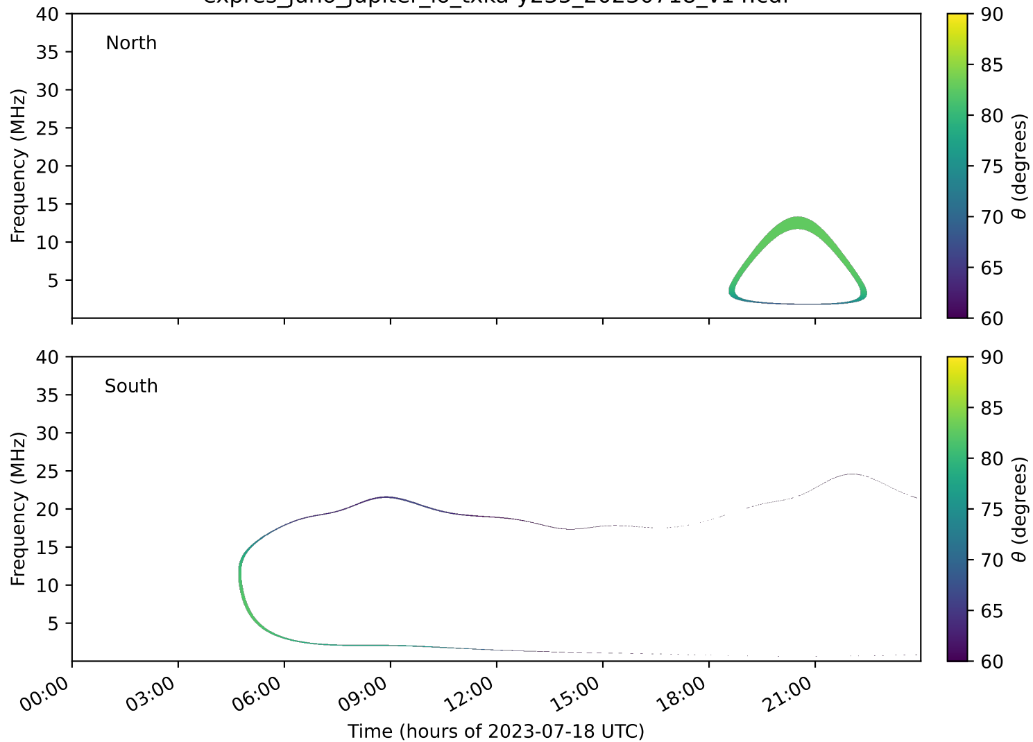
expres_juno_jupiter_io_txka-y235_20230718_v14.cdf
