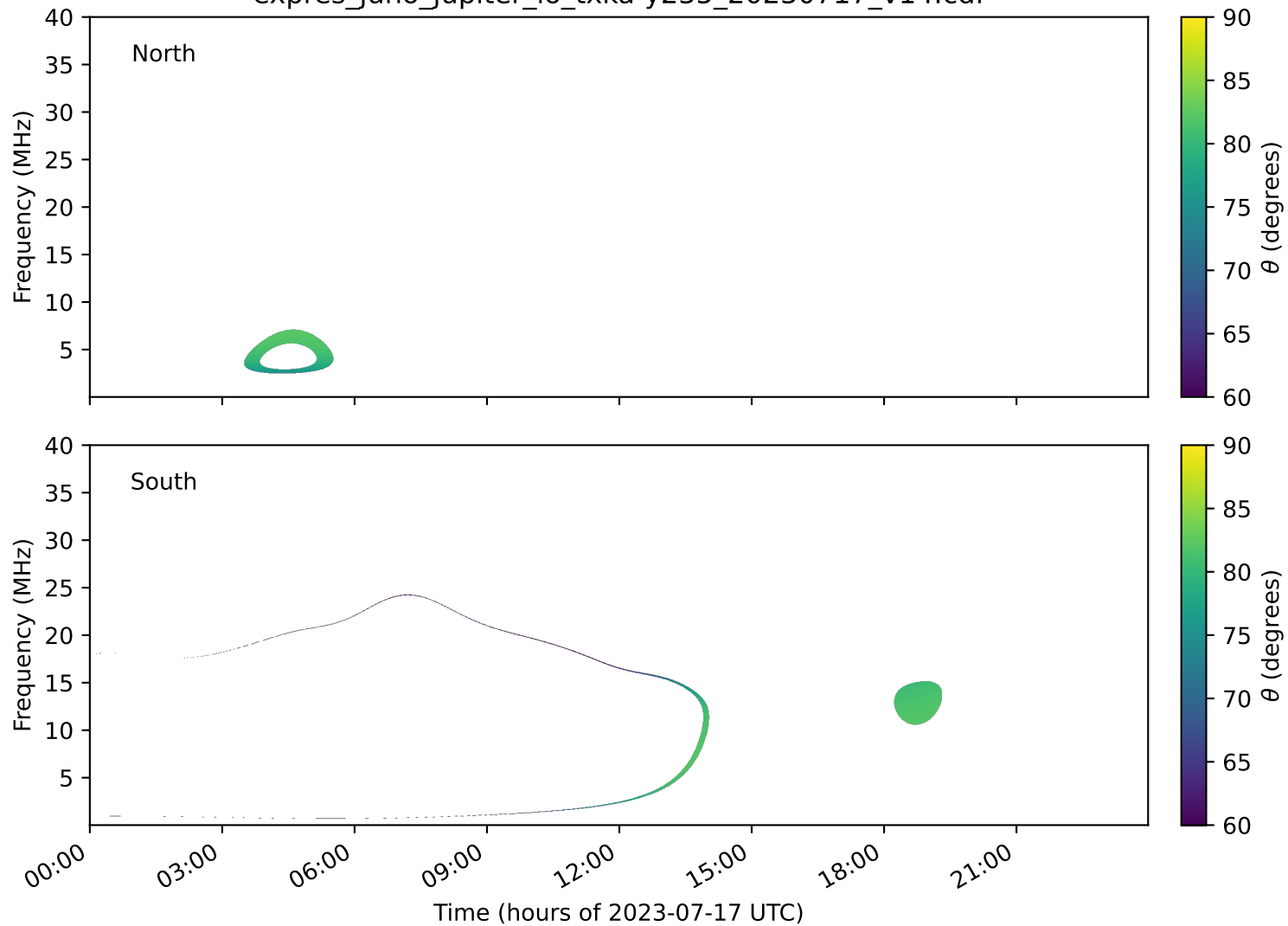
expres_juno_jupiter_io_txka-y235_20230717_v14.cdf
