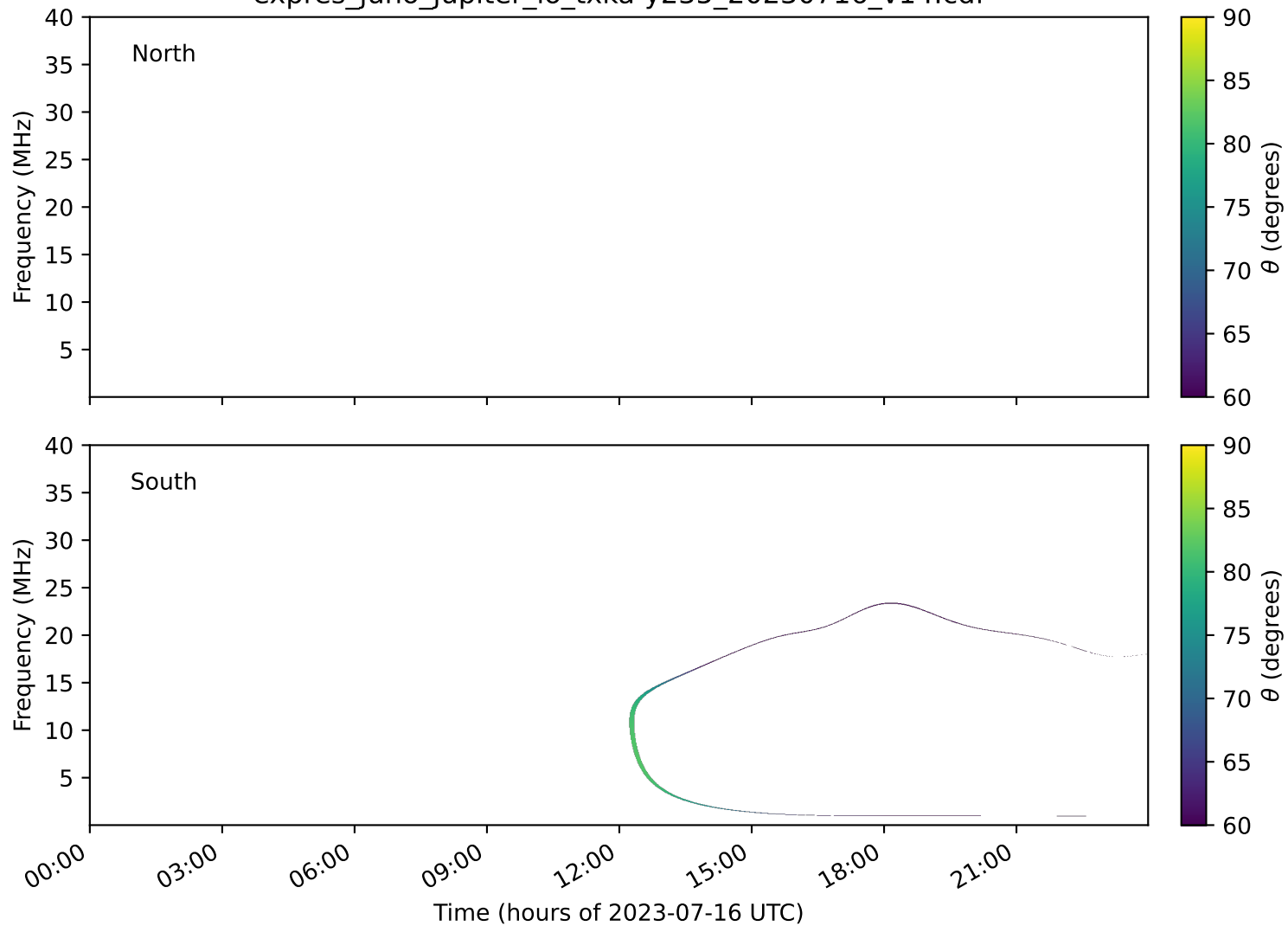
expres_juno_jupiter_io_txka-y235_20230716_v14.cdf
