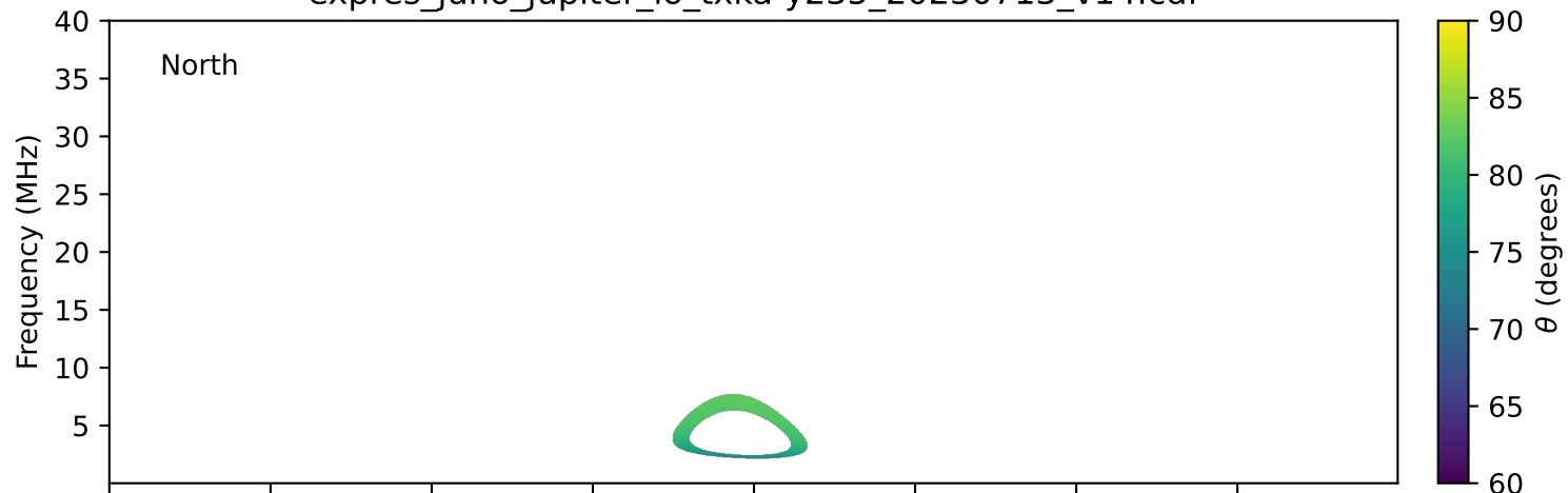
expres_juno_jupiter_io_txka-y235_20230713_v14.cdf
