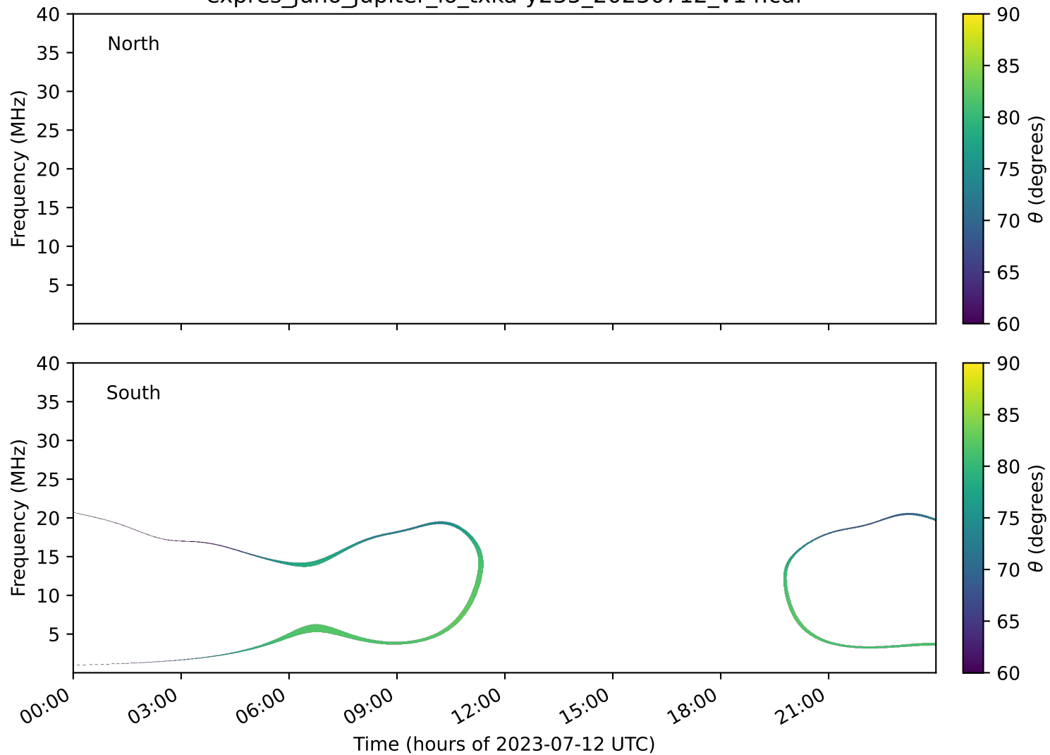
expres_juno_jupiter_io_txka-y235_20230712_v14.cdf
