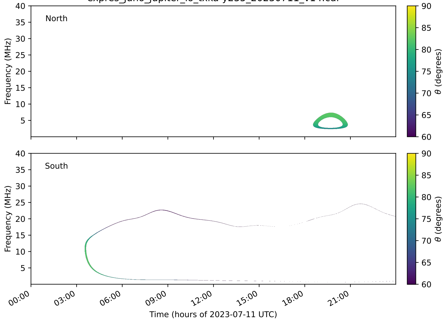
expres_juno_jupiter_io_txka-y235_20230711_v14.cdf
