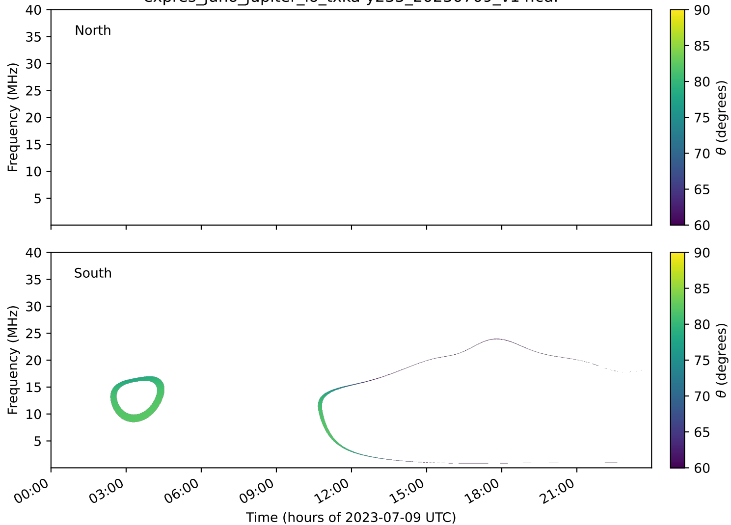
expres_juno_jupiter_io_txka-y235_20230709_v14.cdf
