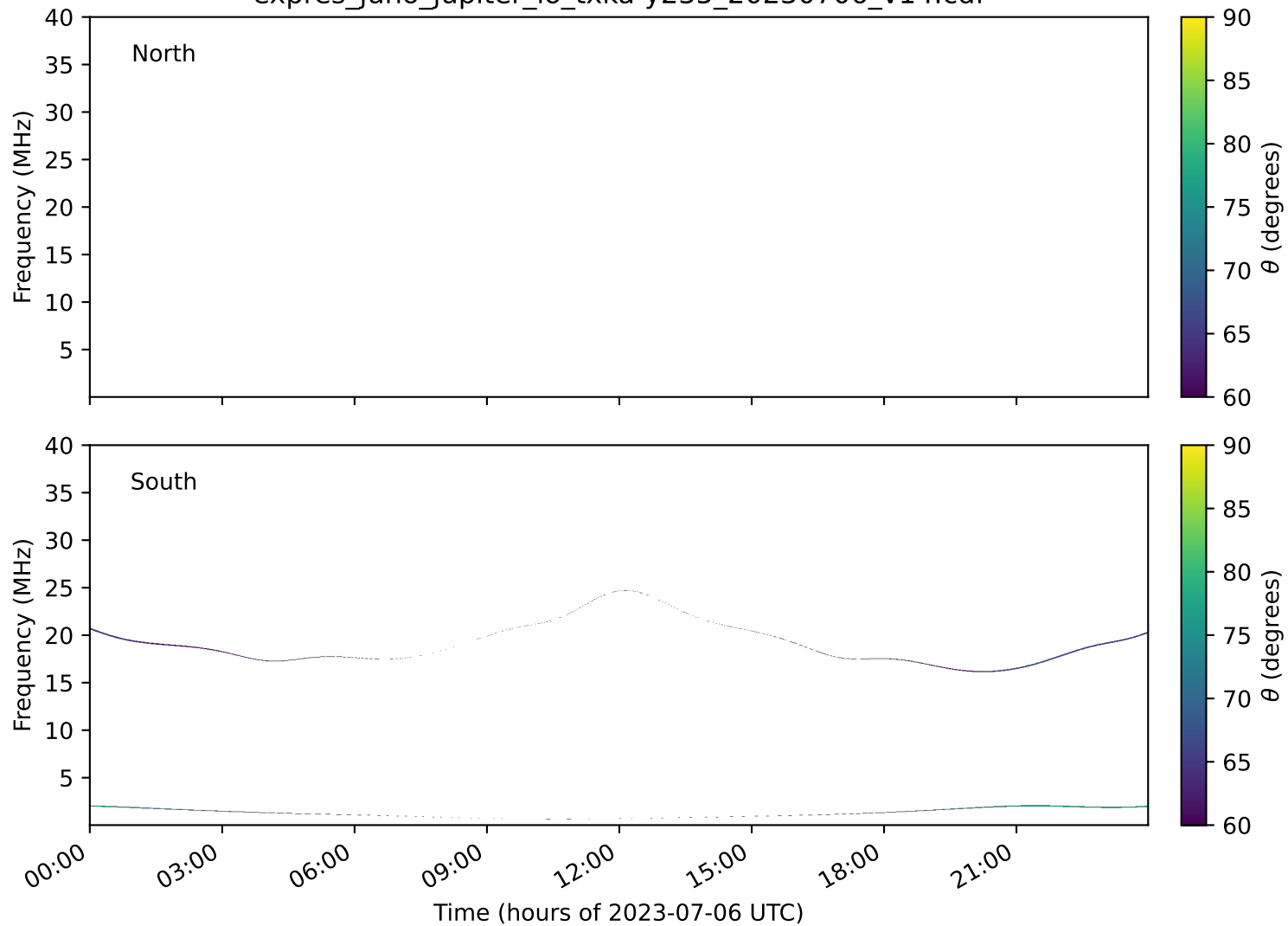
expres_juno_jupiter_io_txka-y235_20230706_v14.cdf
