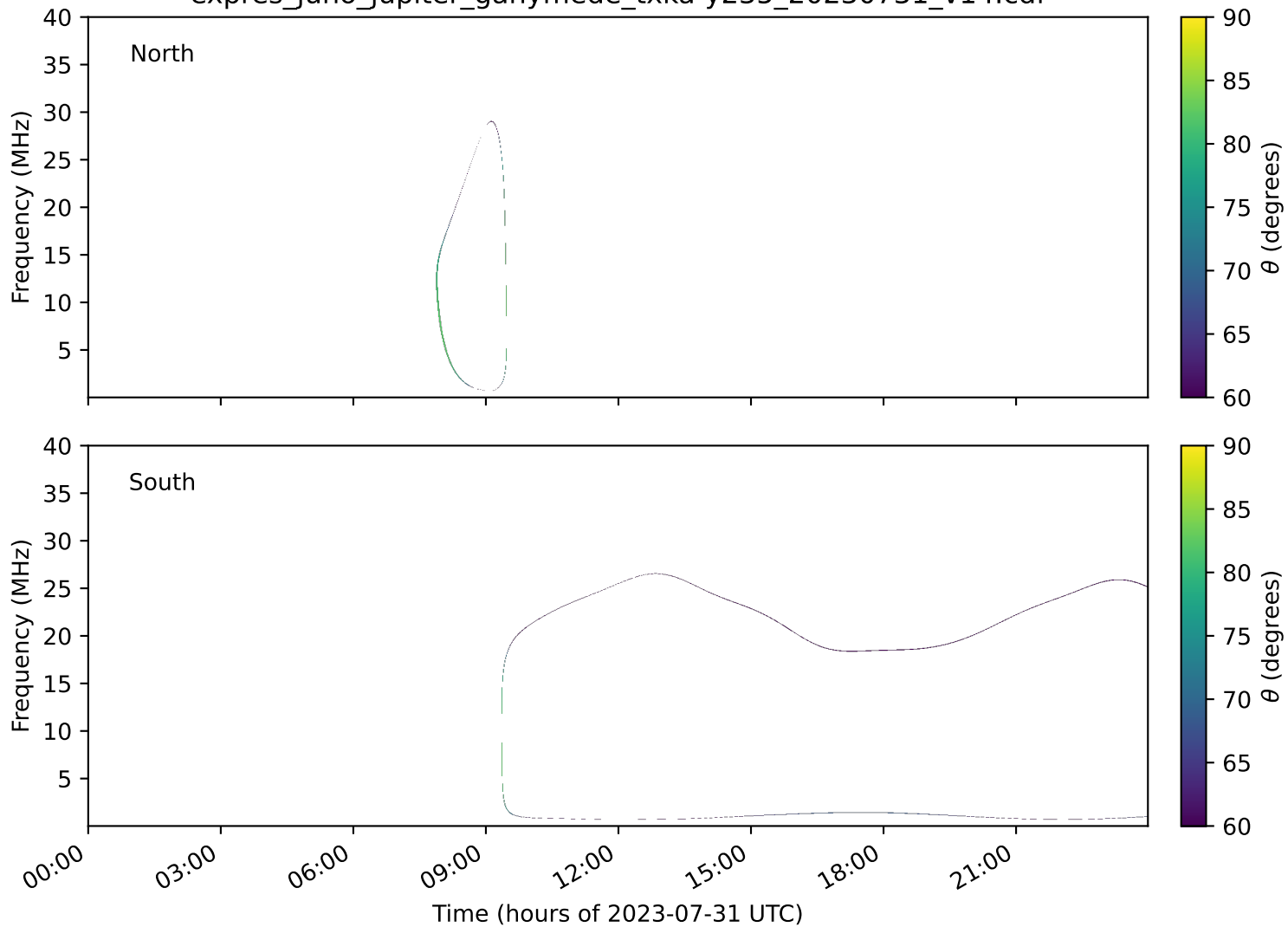
expres_juno_jupiter_ganymede_txka-y235_20230731_v14.cdf
