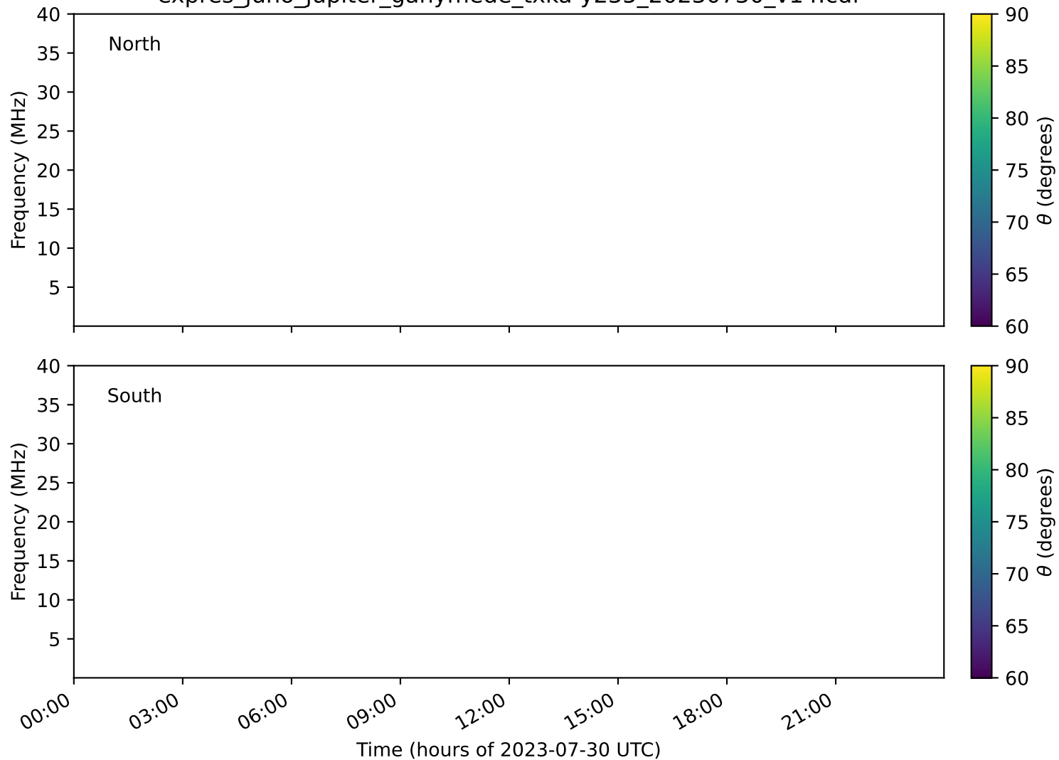
expres_juno_jupiter_ganymede_txka-y235_20230730_v14.cdf
