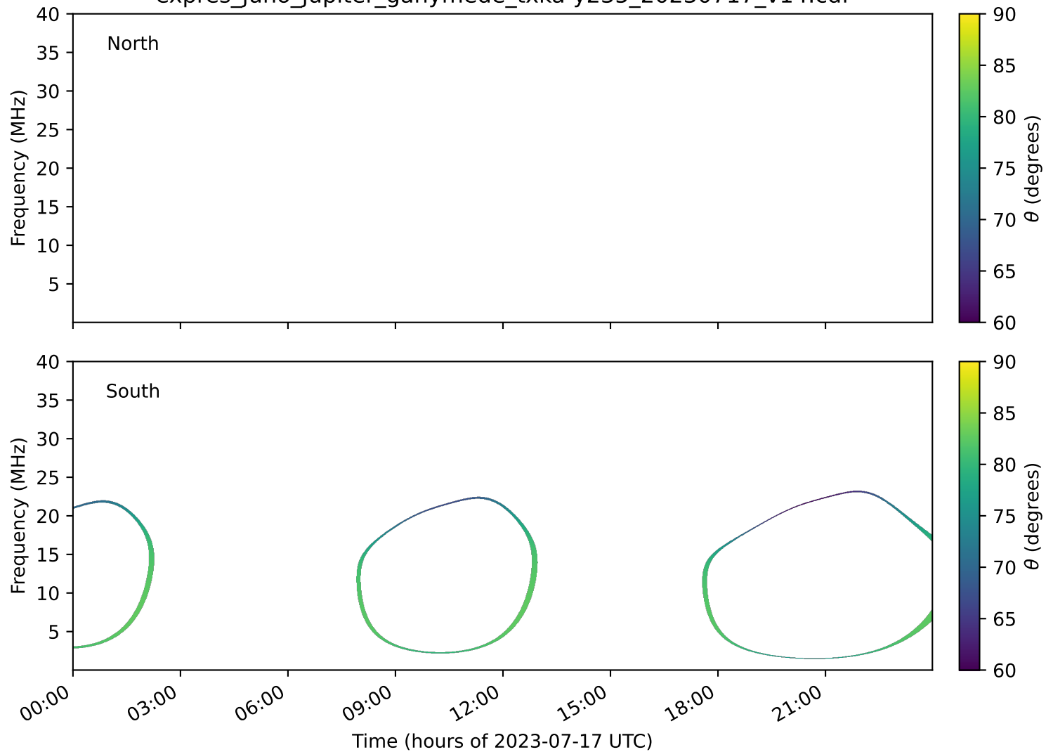
expres_juno_jupiter_ganymede_txka-y235_20230717_v14.cdf
