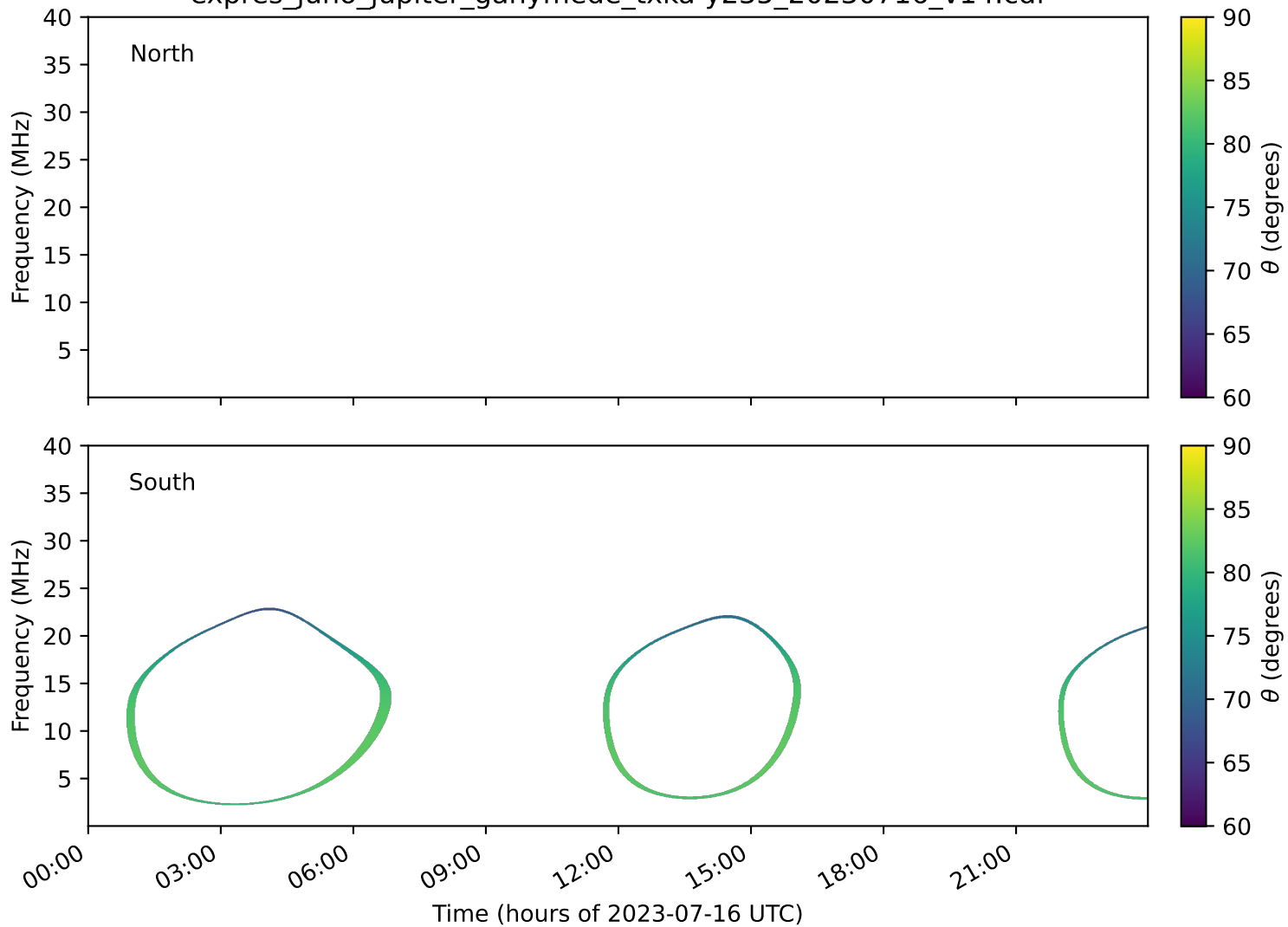
expres_juno_jupiter_ganymede_txka-y235_20230716_v14.cdf
