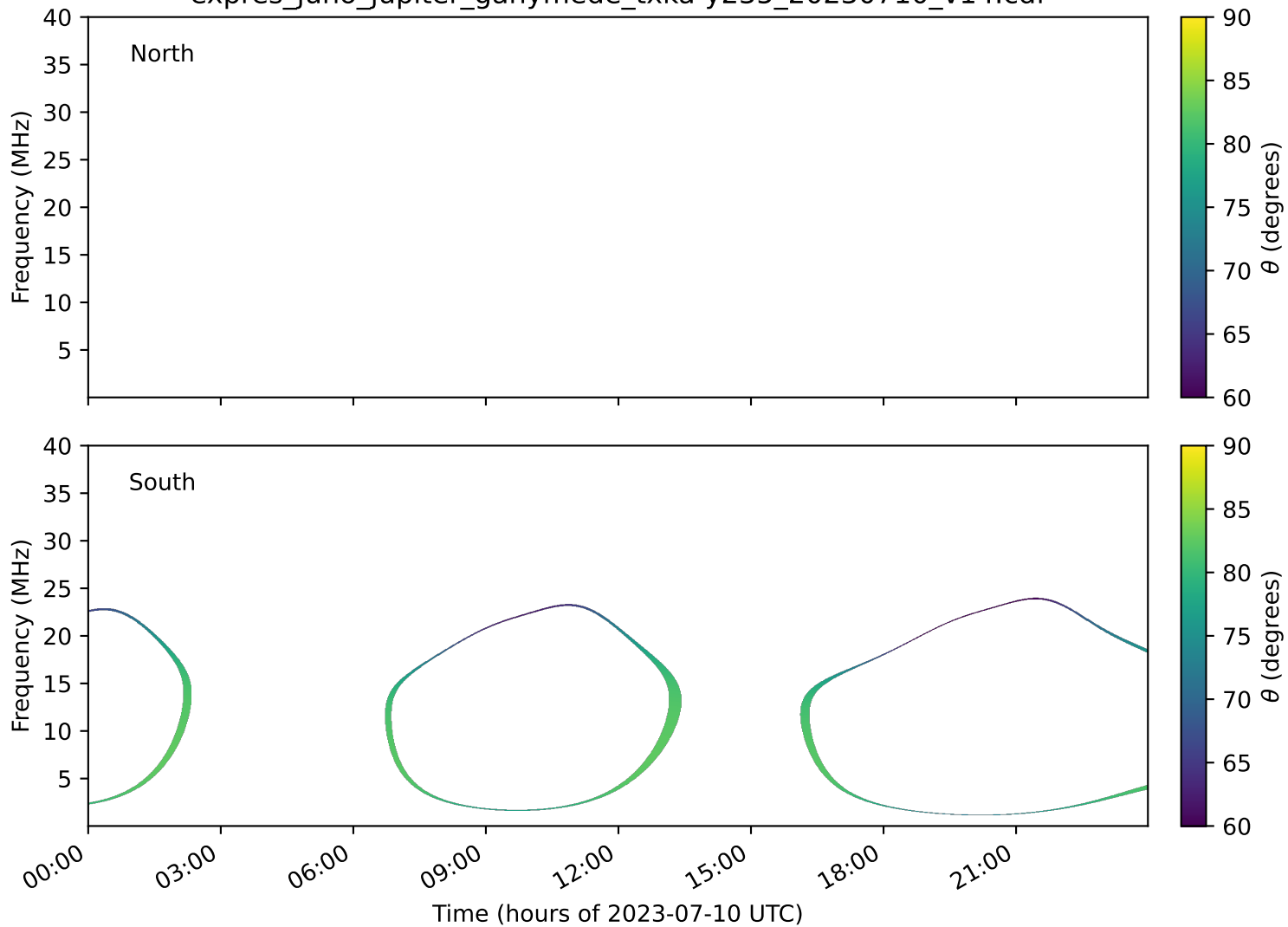
expres_juno_jupiter_ganymede_txka-y235_20230710_v14.cdf
