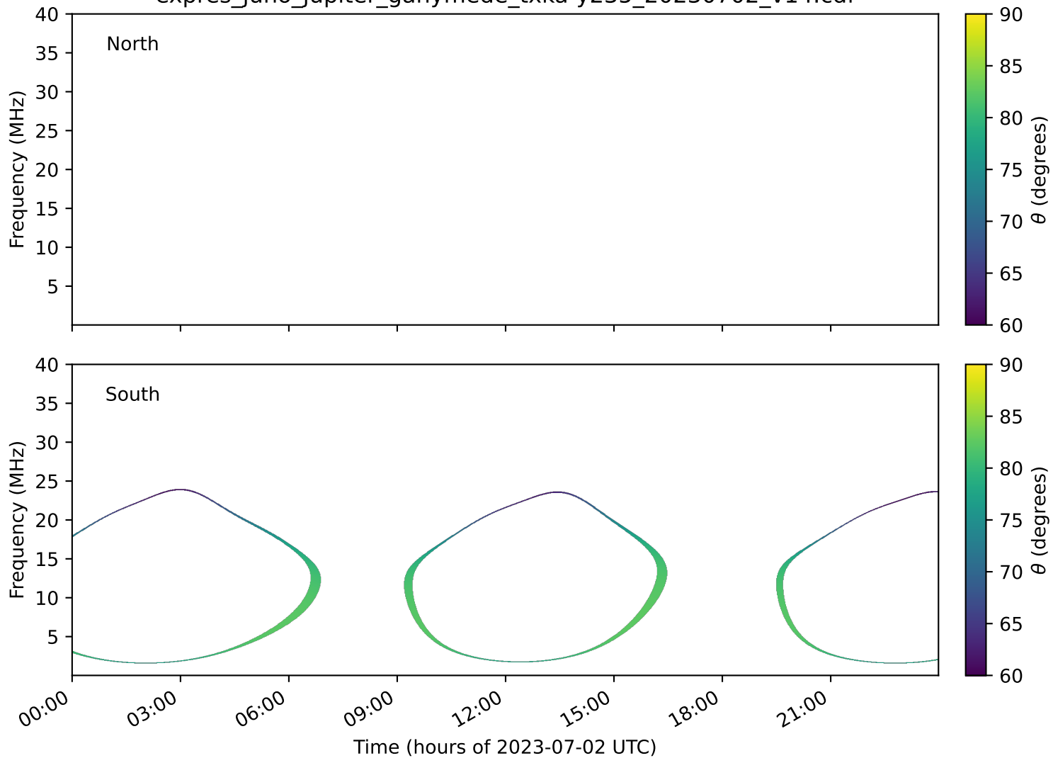
expres_juno_jupiter_ganymede_txka-y235_20230702_v14.cdf
