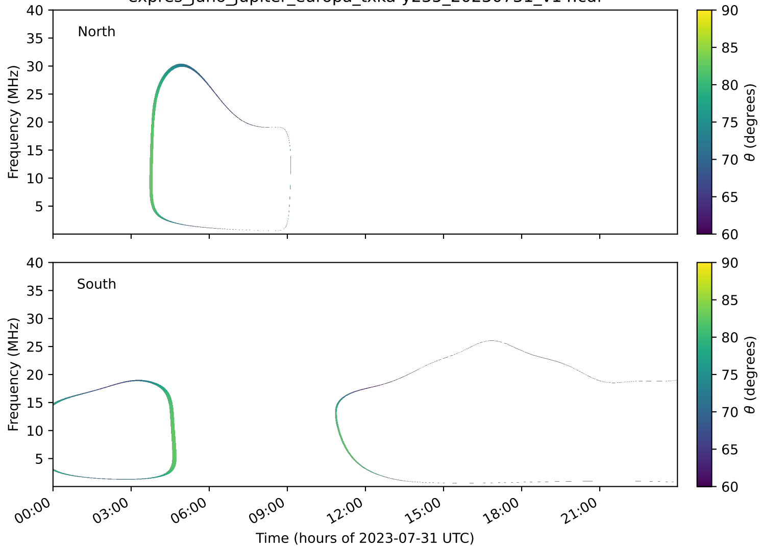
expres_juno_jupiter_europa_txka-y235_20230731_v14.cdf
