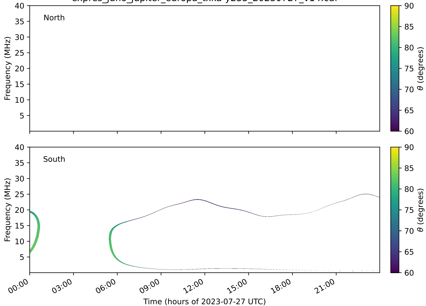
expres_juno_jupiter_europa_txka-y235_20230727_v14.cdf
