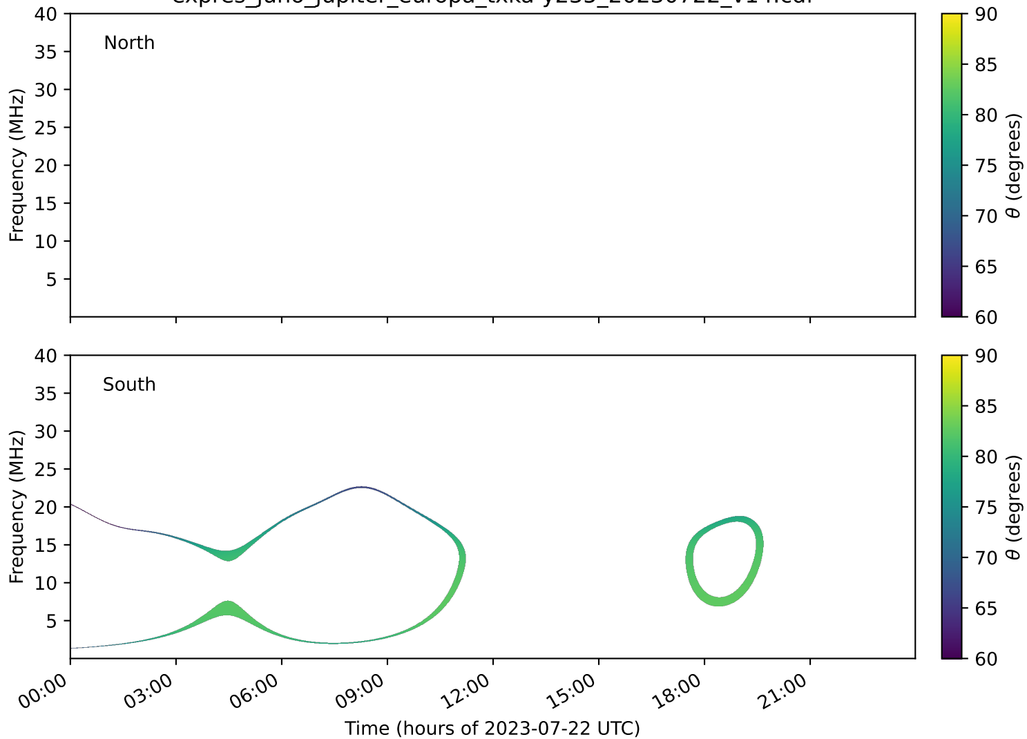
expres_juno_jupiter_europa_txka-y235_20230722_v14.cdf
