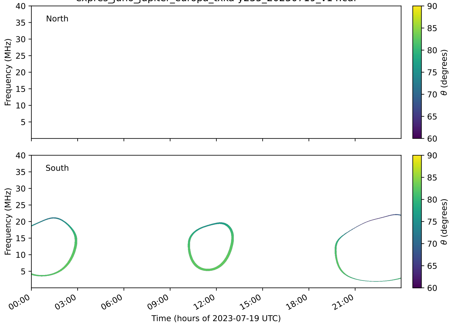
expres_juno_jupiter_europa_txka-y235_20230719_v14.cdf
