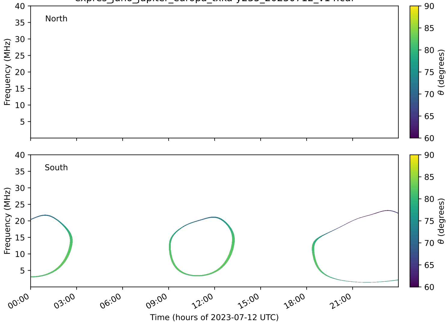
expres_juno_jupiter_europa_txka-y235_20230712_v14.cdf
