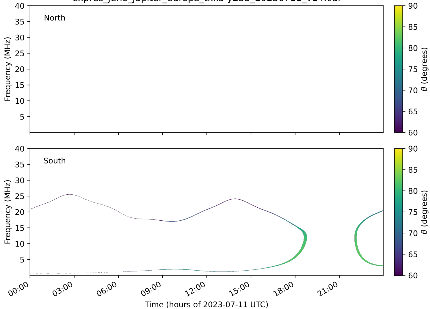
expres_juno_jupiter_europa_txka-y235_20230711_v14.cdf
