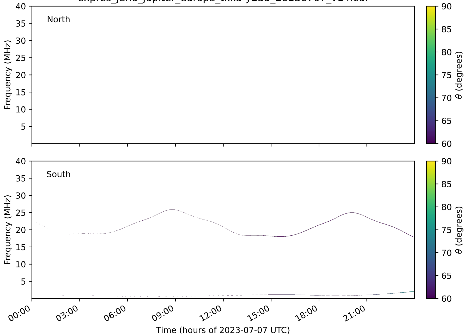
expres_juno_jupiter_europa_txka-y235_20230707_v14.cdf
